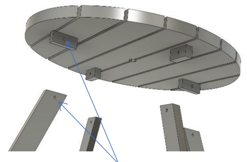
Line these holes up
